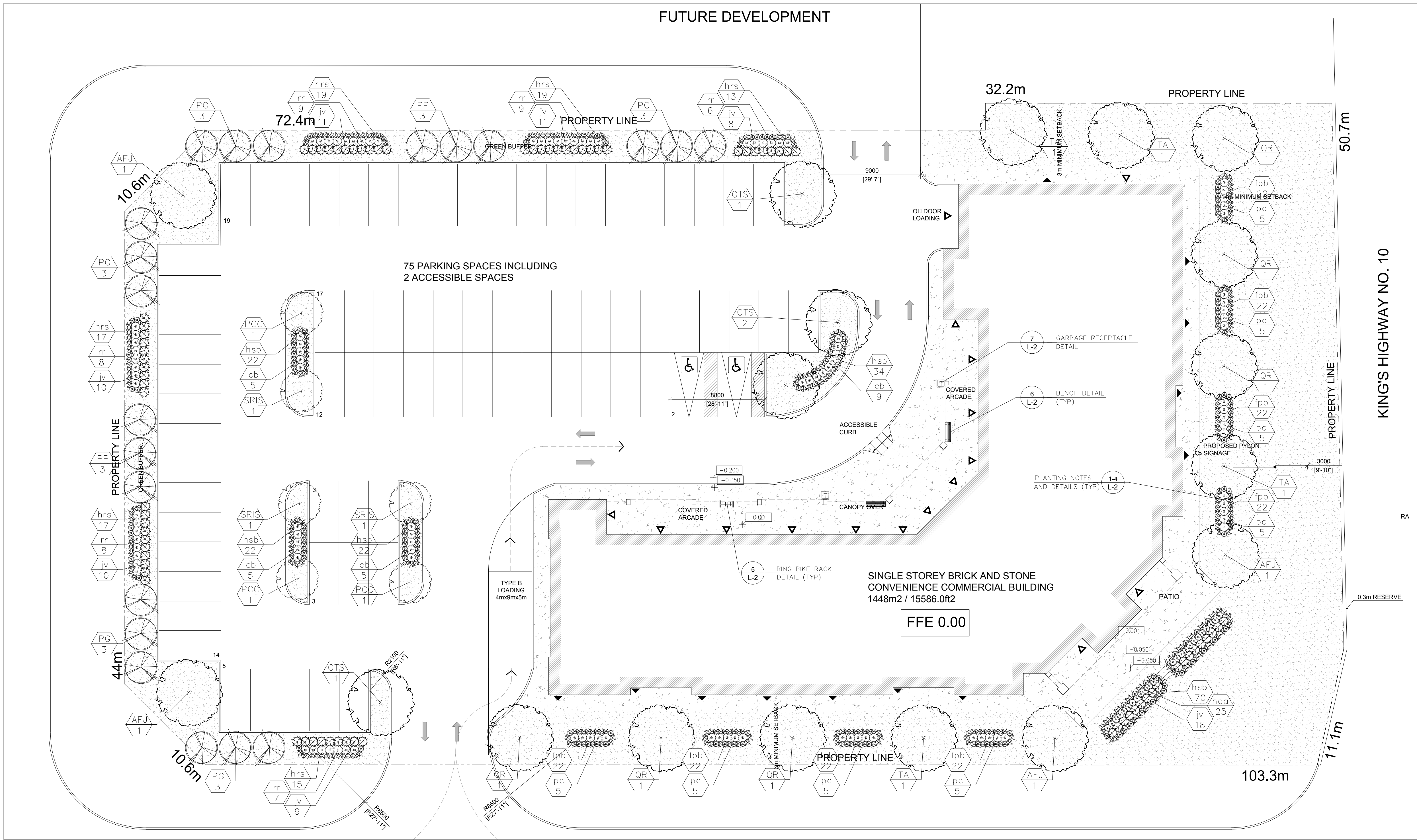
1 Landscape Plan L-1 Scale 1:200
